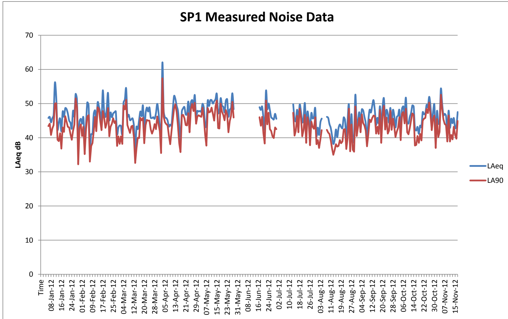
Figure A1 Surrogate baseline noise levels (2012) at location P1
