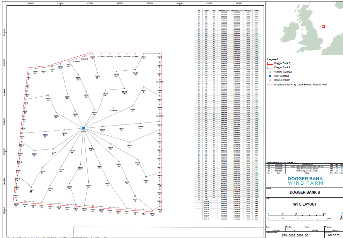
Figure 2: Dogger Bank B OWF IA Cable Layout
