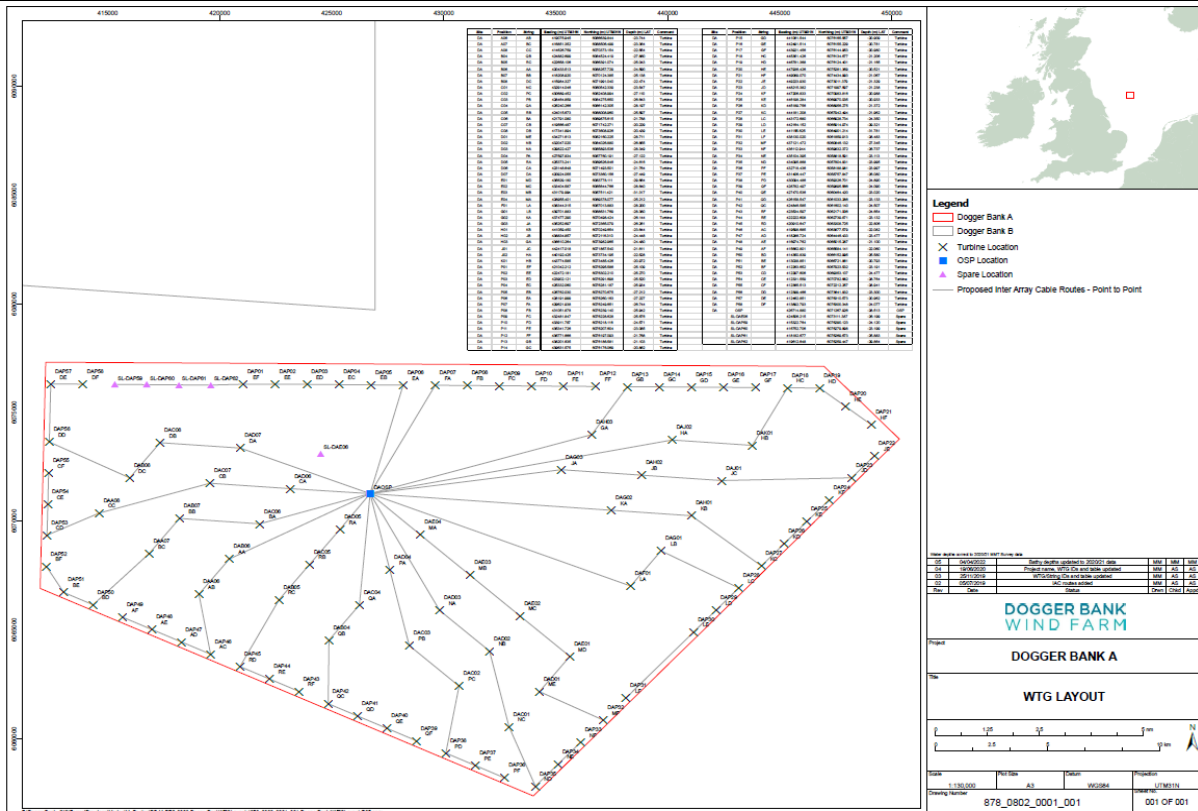
Figure 1: Dogger Bank A OWF IA Cable Layout
