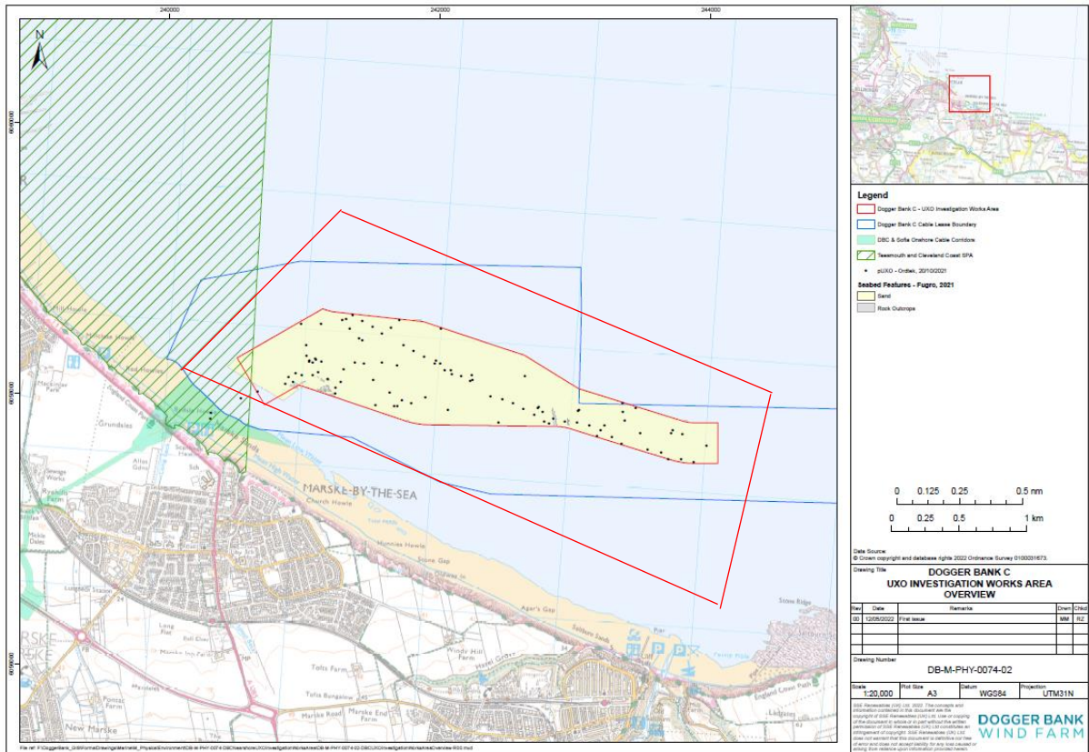
Figure 3: Dogger Bank C Nearshore Area
