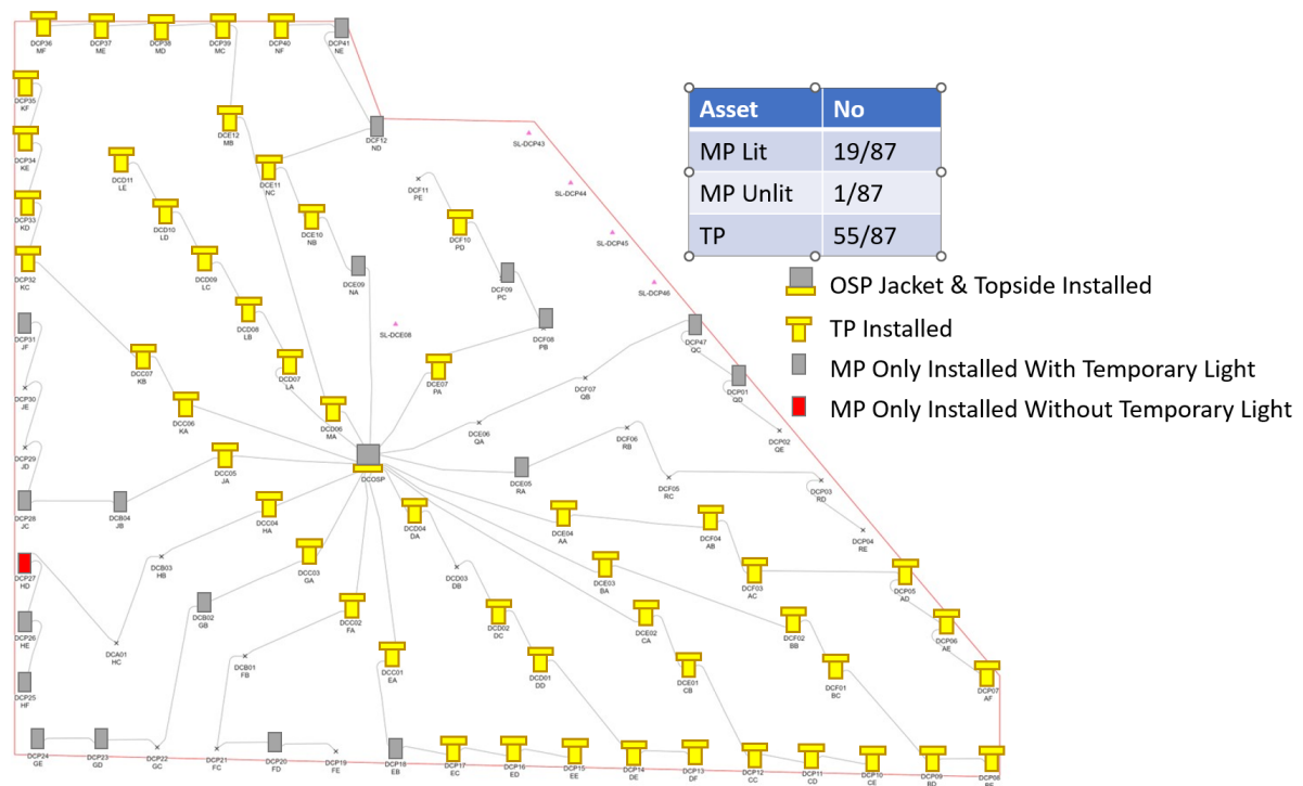
Figure 1: Dogger Bank C OWF Foundation Installation
