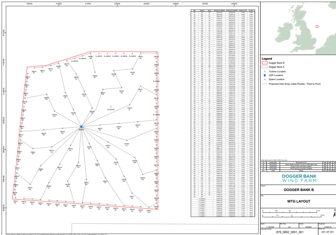
Figure 1: General Location of Dogger Bank B Offshore Construction Area
